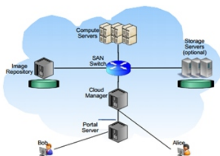
Fig 2:cloud architecture
