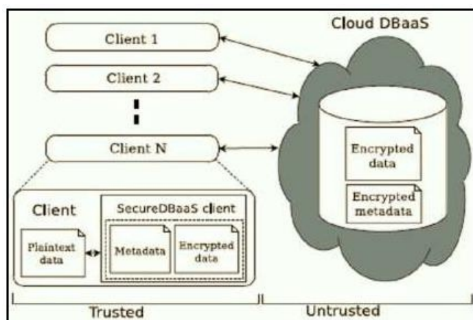
Fig.1. SecureDBaaS Architecture.
