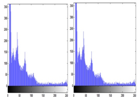
Fig.7 Histograms of original and decrypted image
