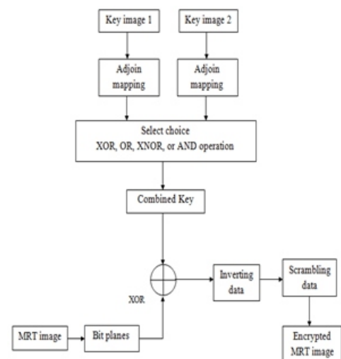
Fig3. Block diagram of AM algorithm
