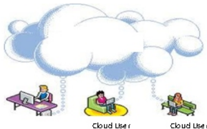
Fig 1: Cloud Architecture
