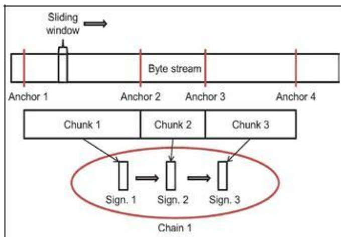
Fig. 1: From Stream to Chain
