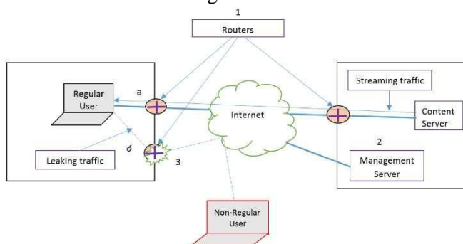
Fig 1.0 System Architecture
