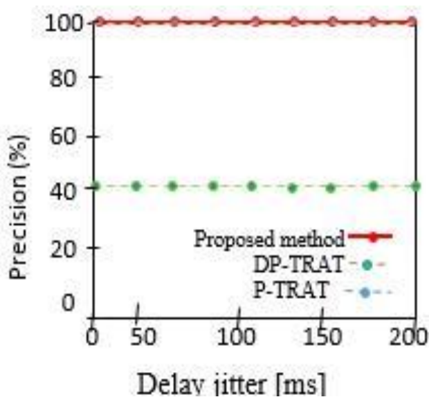
Fig. 5.1.1 Accuracy
